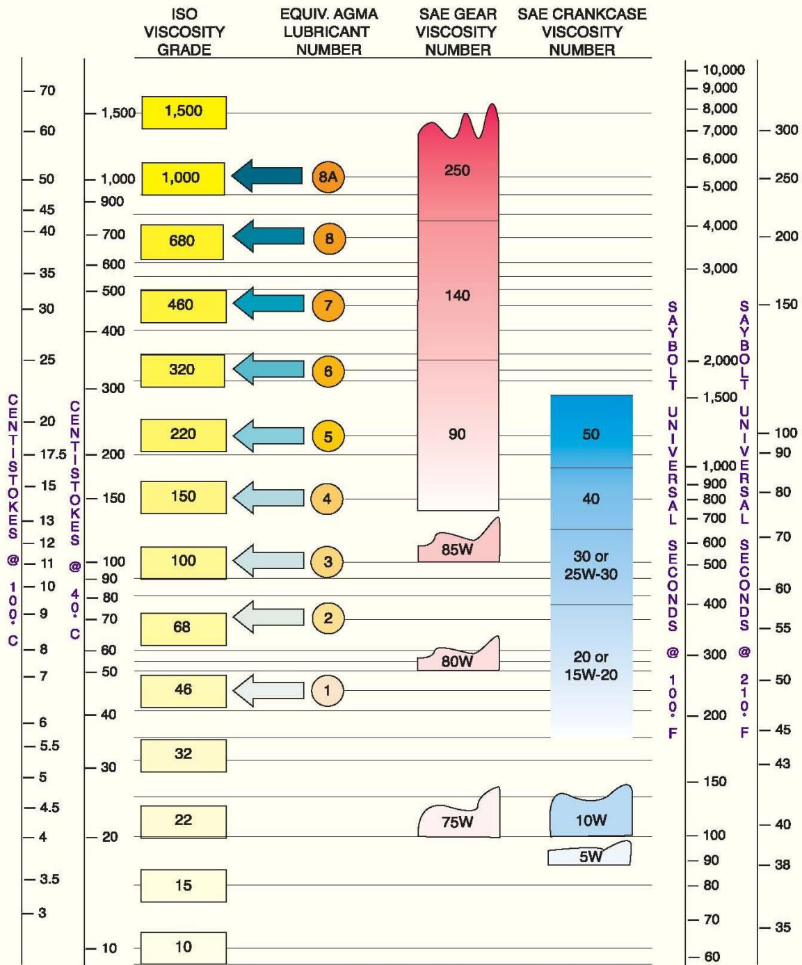
VISCOSITIES AT VARIOUS TEMPERATURES ASSUME 95 VI OILS Note: Viscosities at various temperatures are related horizontally. SAE gear and crankcase specifications are at 100°C only.
